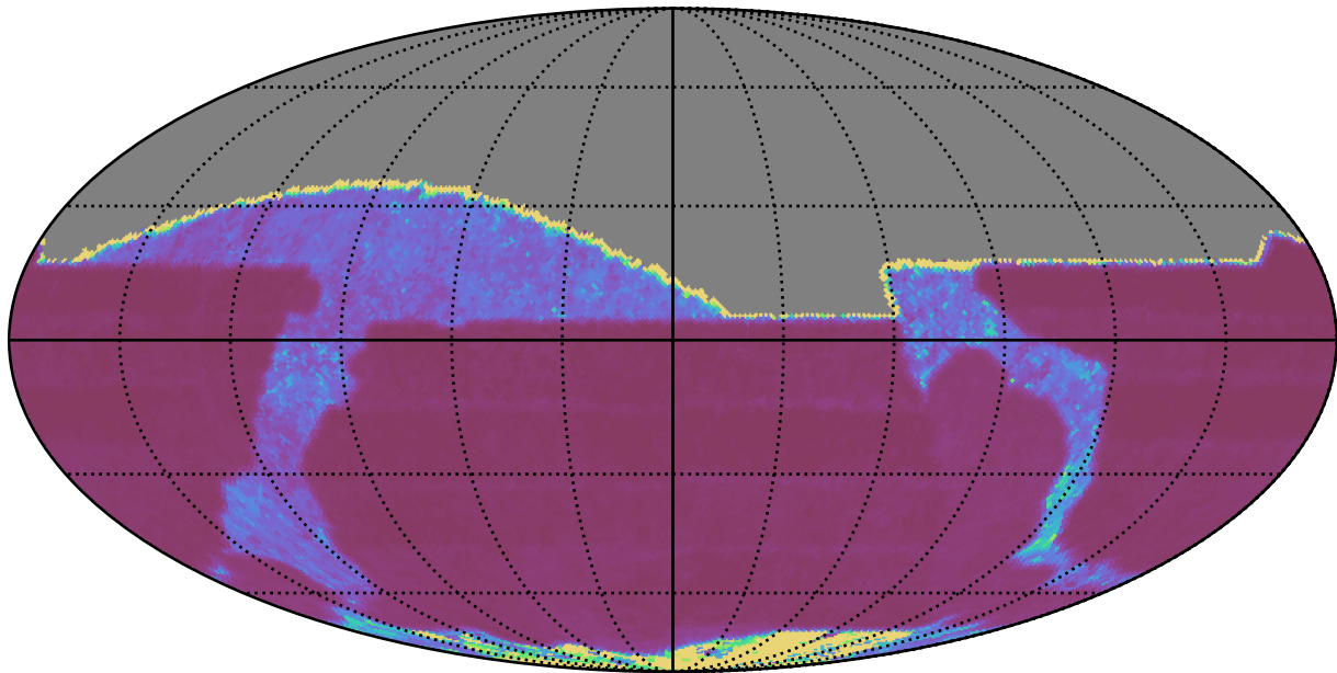
no_high_blob_v3.3_10yrs All sky r band: Median Inter-Night Gap
