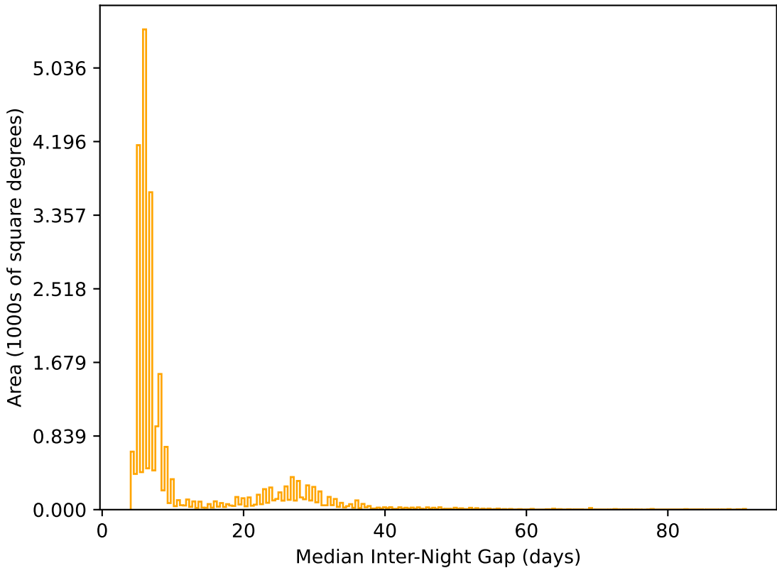
no_high_blob_v3.3_10yrs All sky r band: Median Inter-Night Gap
