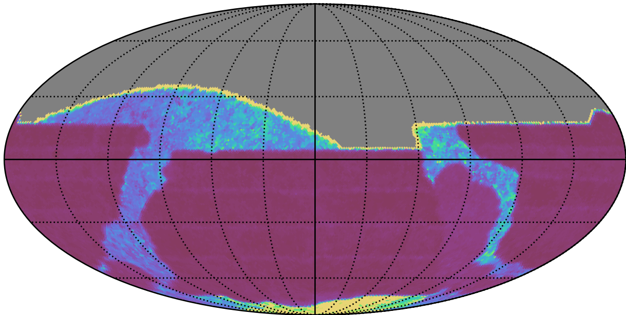
no_high_blob_v3.3_10yrs All sky i band: Median Inter-Night Gap
