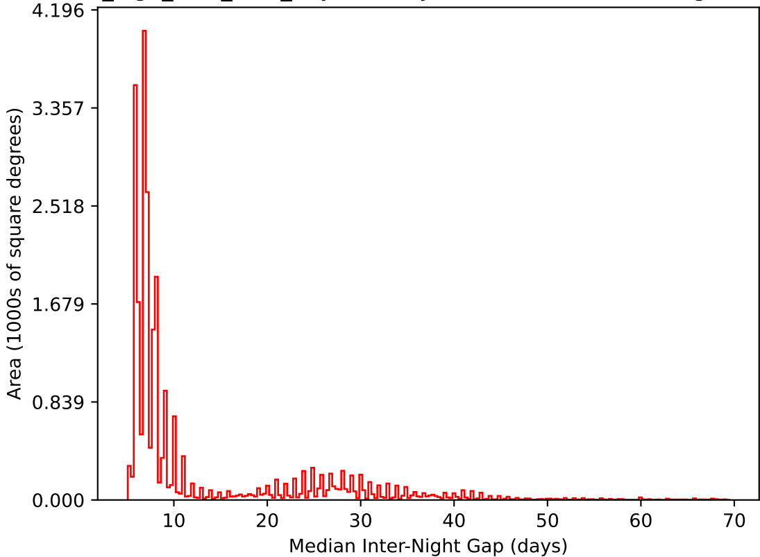
no_high_blob_v3.3_10yrs All sky i band: Median Inter-Night Gap
