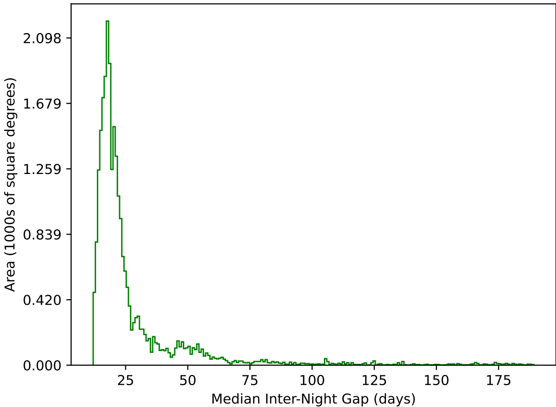
no_high_blob_v3.3_10yrs All sky g band: Median Inter-Night Gap
