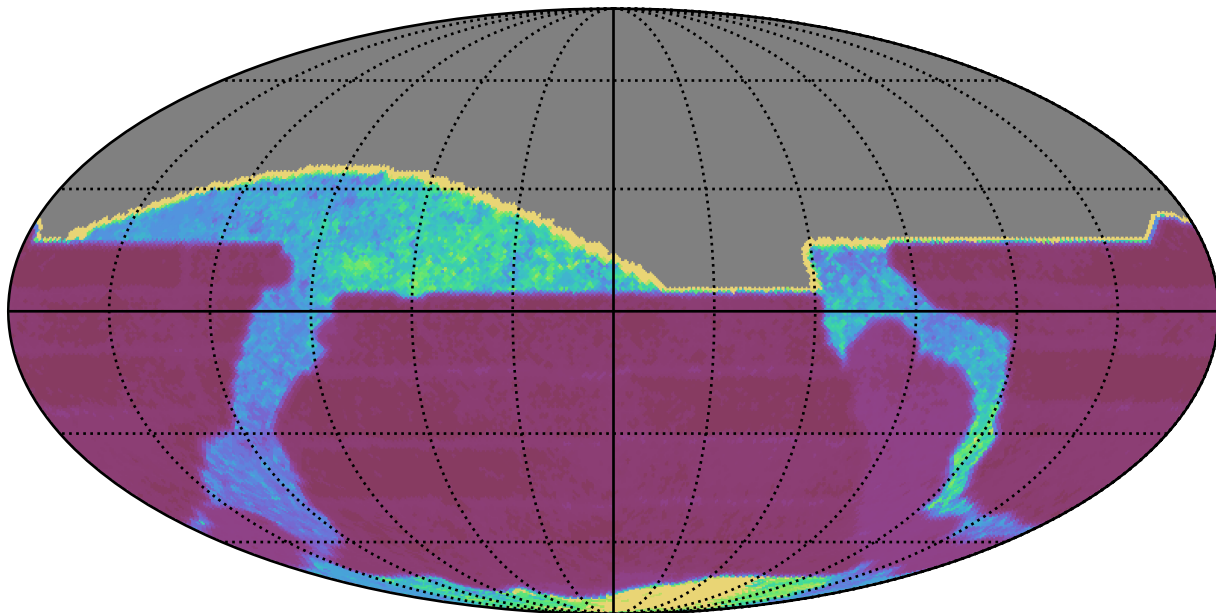
no_high_blob_v3.3_10yrs All sky all bands: Median Inter-Night Gap
