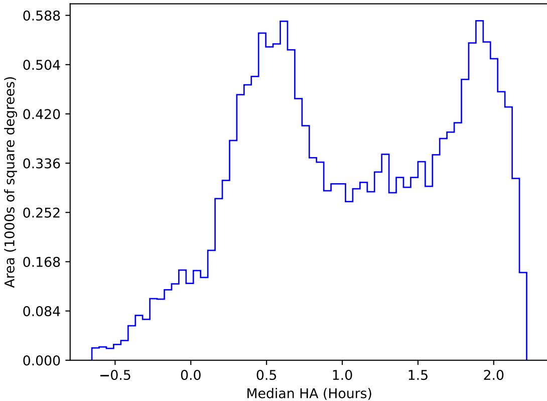
no_high_blob_v3.3_10yrs WFD z band: Median HA
