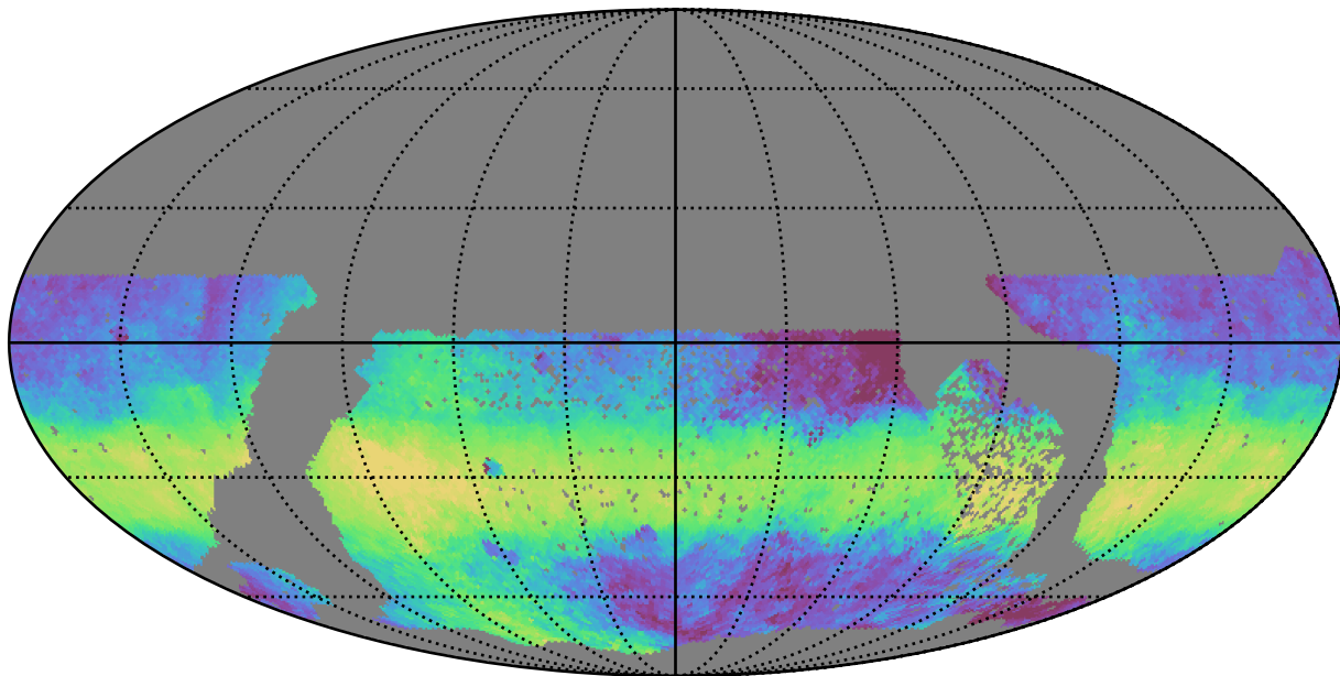
no_high_blob_v3.3_10yrs WFD y band: Median HA
