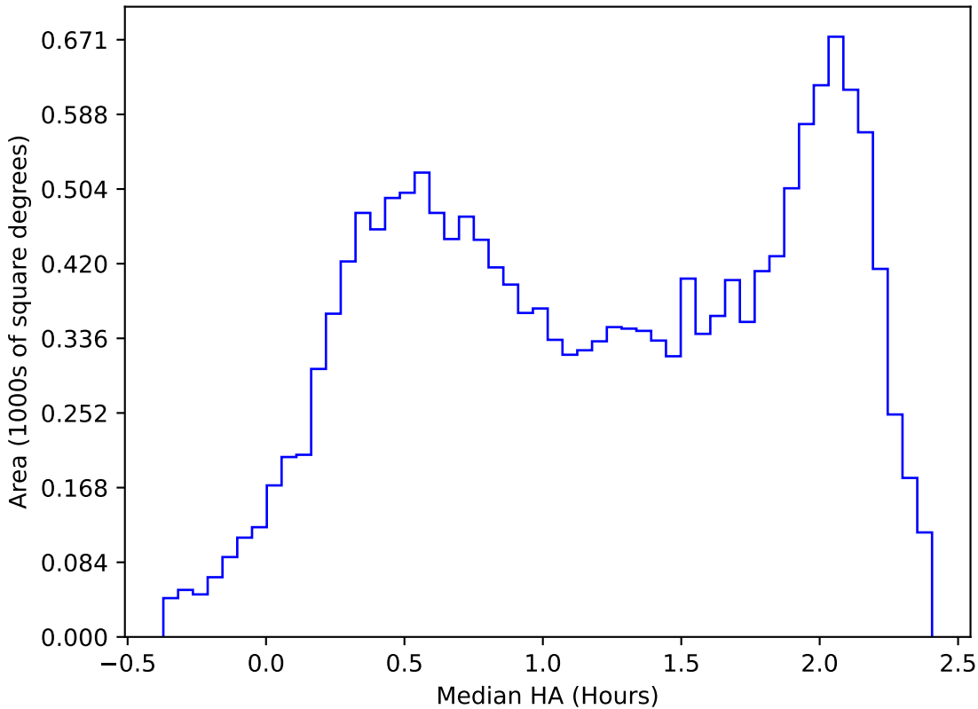
no_high_blob_v3.3_10yrs WFD y band: Median HA
