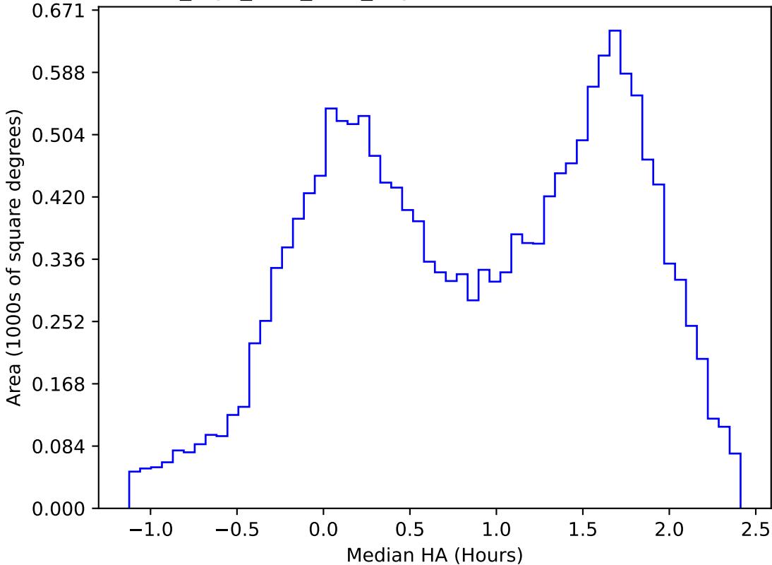
no_high_blob_v3.3_10yrs WFD u band: Median HA
