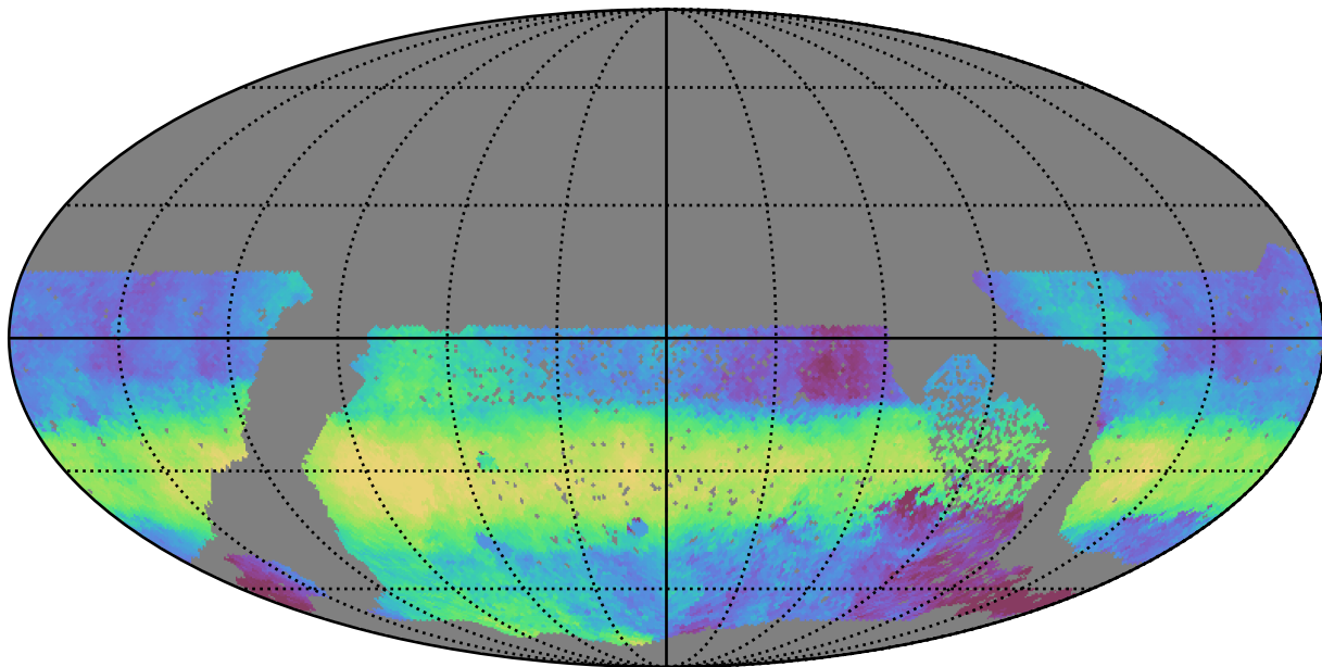
no_high_blob_v3.3_10yrs WFD r band: Median HA
