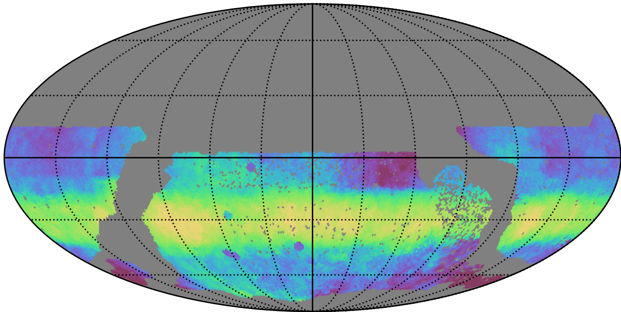
no_high_blob_v3.3_10yrs WFD i band: Median HA
