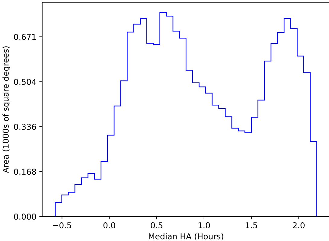
no_high_blob_v3.3_10yrs WFD i band: Median HA
