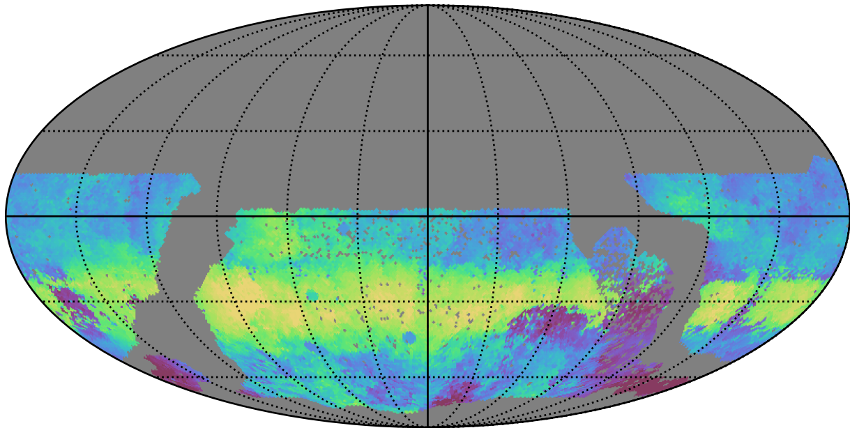
no_high_blob_v3.3_10yrs WFD g band: Median HA
