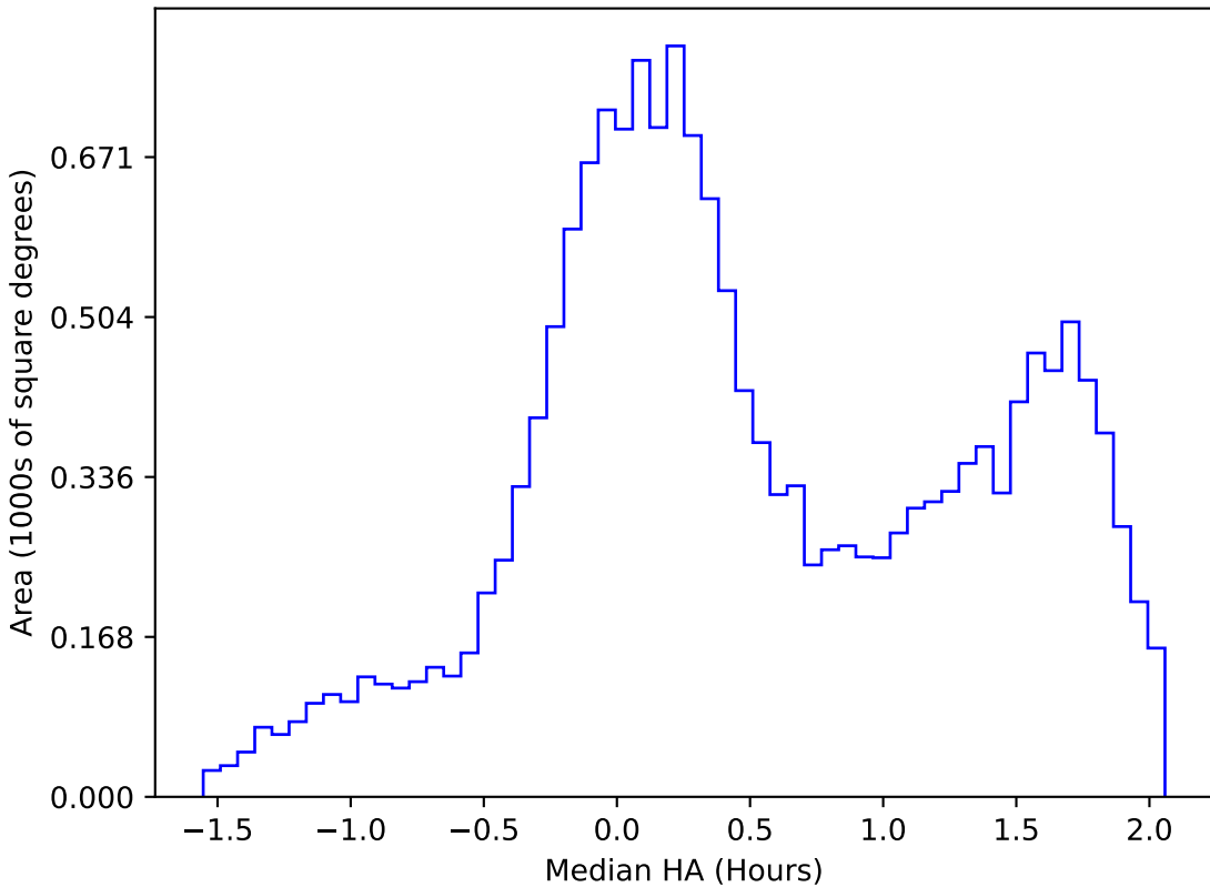
no_high_blob_v3.3_10yrs WFD g band: Median HA
