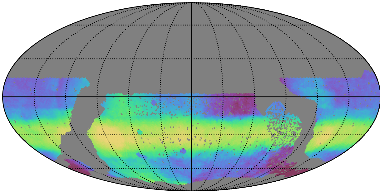
no_high_blob_v3.3_10yrs WFD all bands: Median HA
