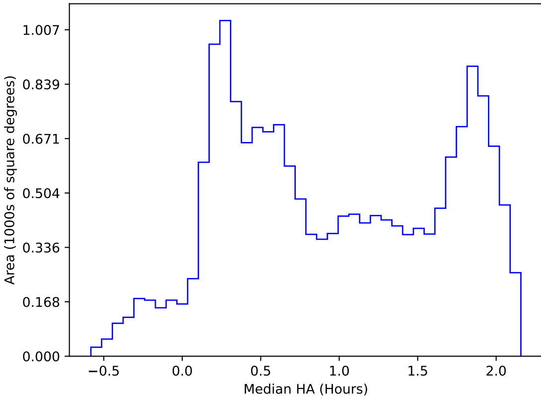
no_high_blob_v3.3_10yrs WFD all bands: Median HA
