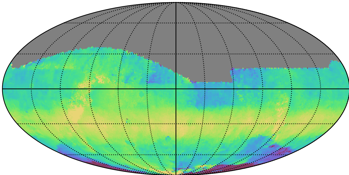
no_high_blob_v3.3_10yrs All sky z band: Median HA
