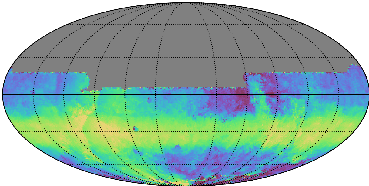
no_high_blob_v3.3_10yrs All sky y band: Median HA
