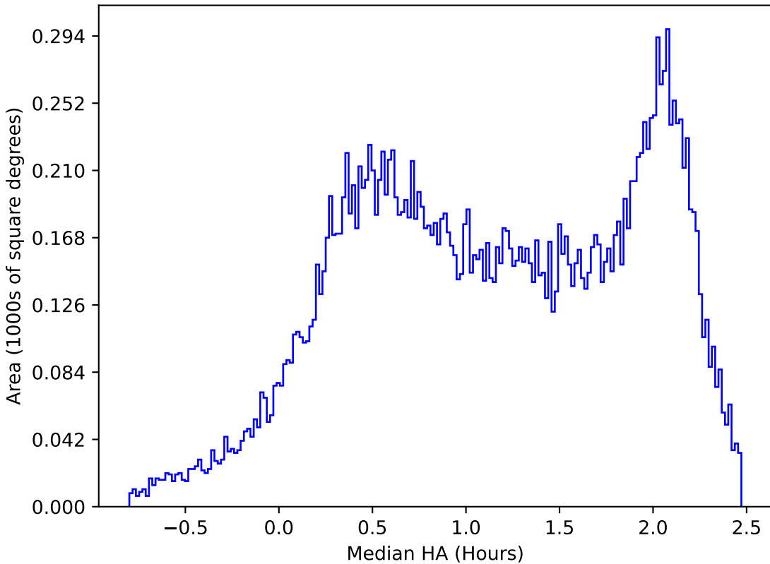
no_high_blob_v3.3_10yrs All sky y band: Median HA
