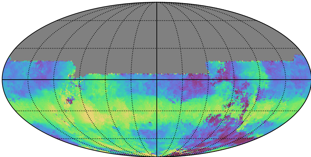
no_high_blob_v3.3_10yrs All sky u band: Median HA
