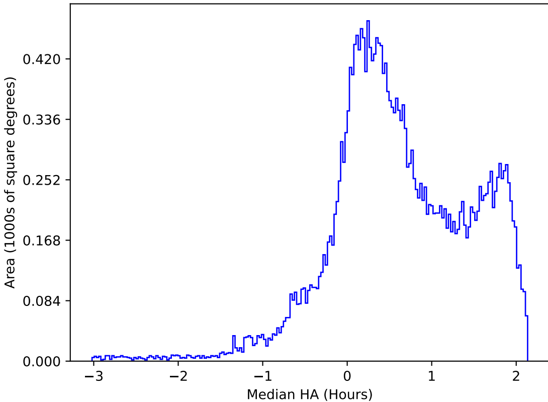
no_high_blob_v3.3_10yrs All sky r band: Median HA
