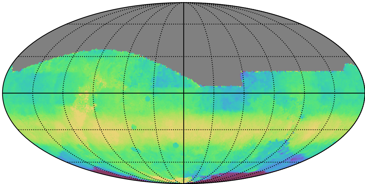
no_high_blob_v3.3_10yrs All sky i band: Median HA
