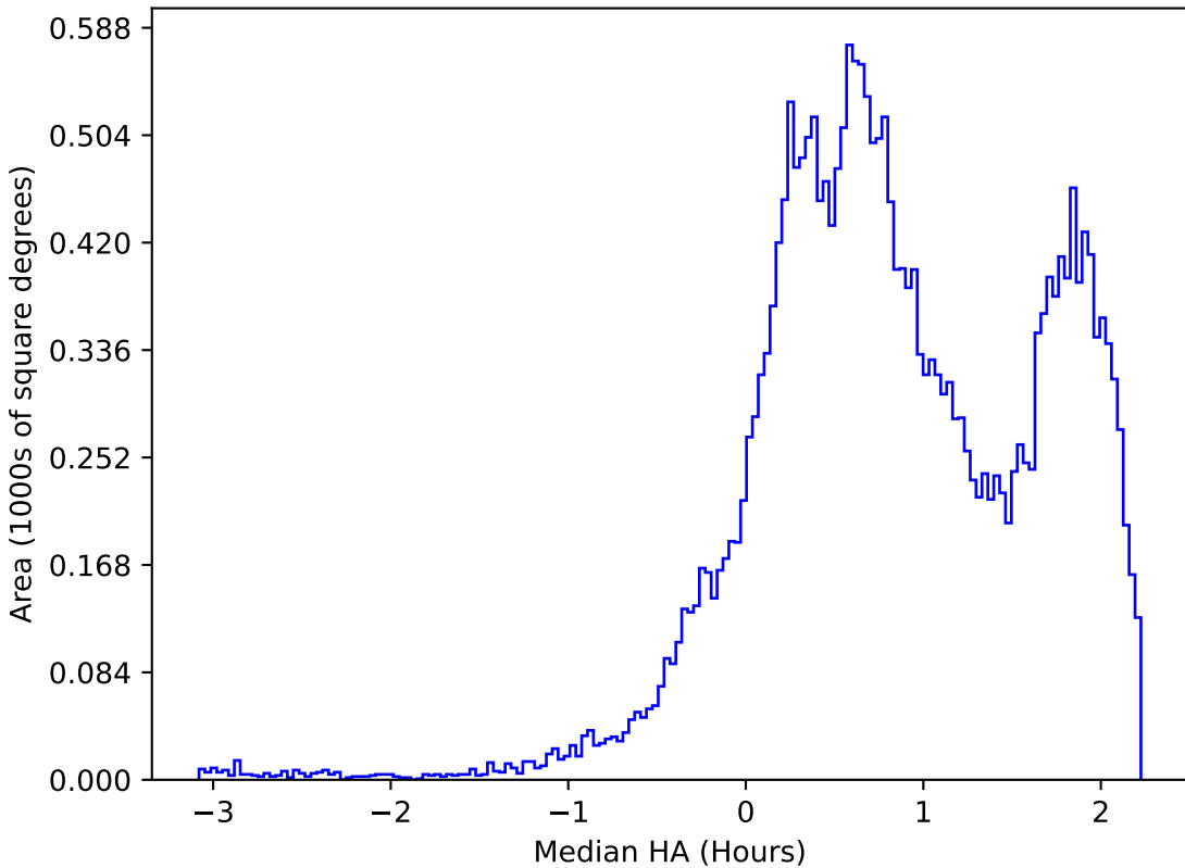
no_high_blob_v3.3_10yrs All sky i band: Median HA
