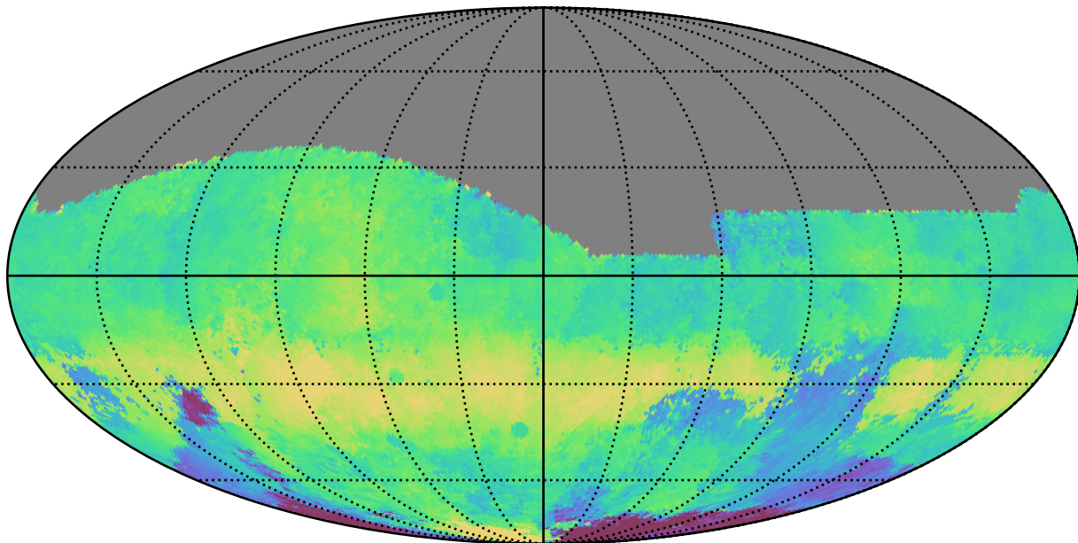
no_high_blob_v3.3_10yrs All sky g band: Median HA
