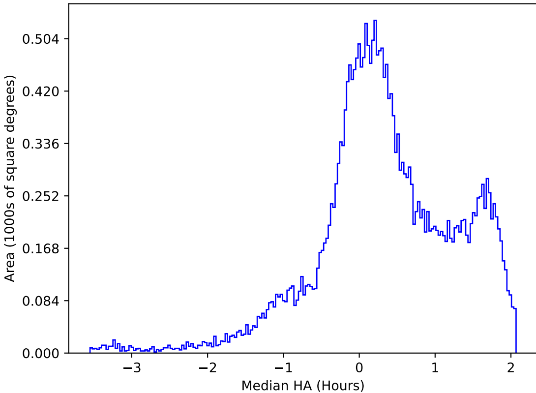
no_high_blob_v3.3_10yrs All sky g band: Median HA
