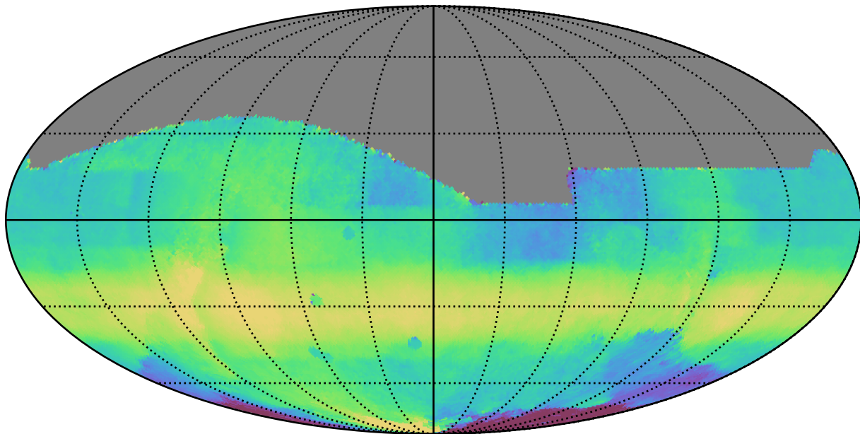
no_high_blob_v3.3_10yrs All sky all bands: Median HA
