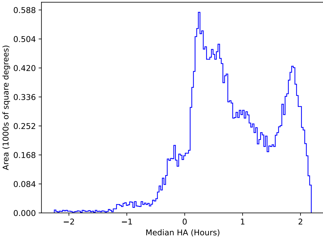
no_high_blob_v3.3_10yrs All sky all bands: Median HA
