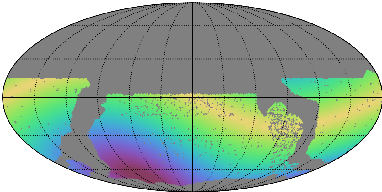
no_high_blob_v3.3_10yrs WFD z band: Max solarElong
