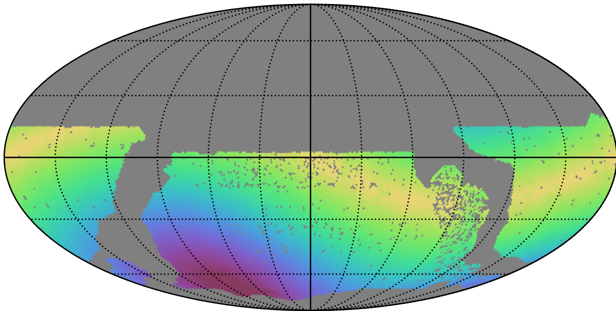
no_high_blob_v3.3_10yrs WFD u band: Max solarElong
