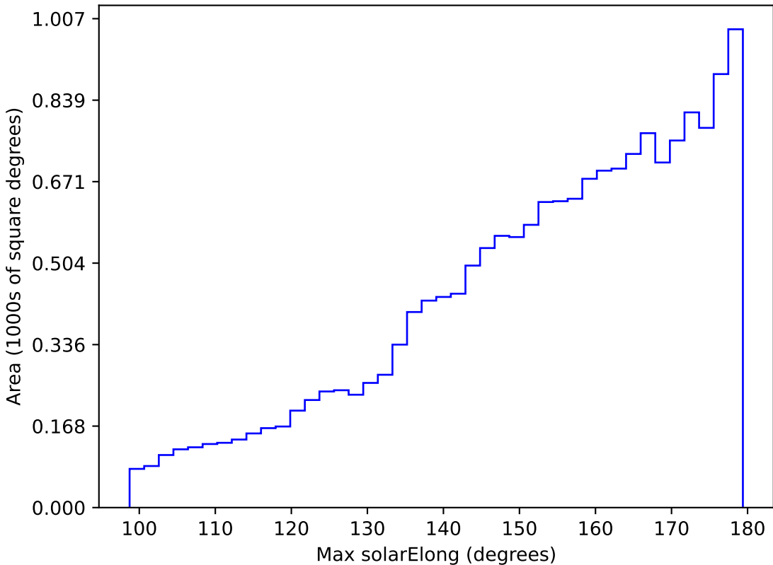
no_high_blob_v3.3_10yrs WFD r band: Max solarElong
