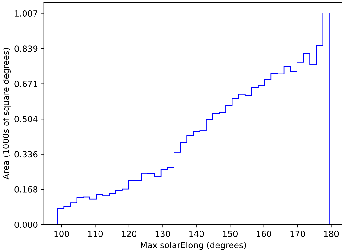
no_high_blob_v3.3_10yrs WFD i band: Max solarElong
