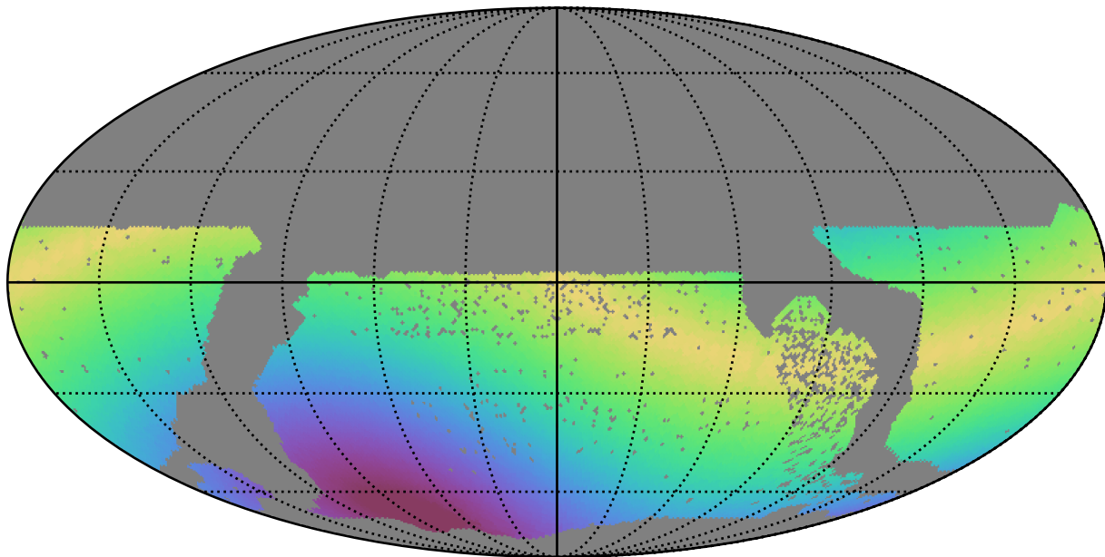
no_high_blob_v3.3_10yrs WFD g band: Max solarElong
