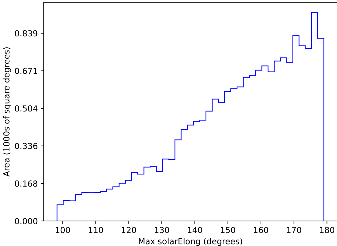
no_high_blob_v3.3_10yrs WFD g band: Max solarElong
