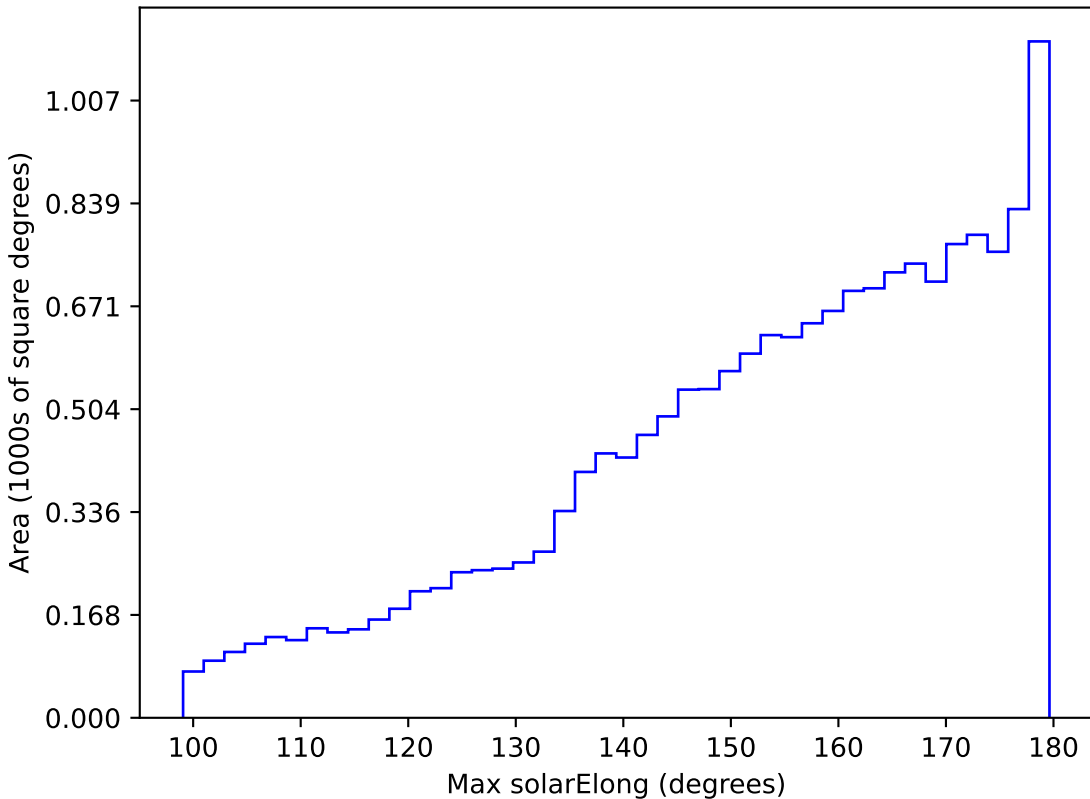
no_high_blob_v3.3_10yrs WFD all bands: Max solarElong
