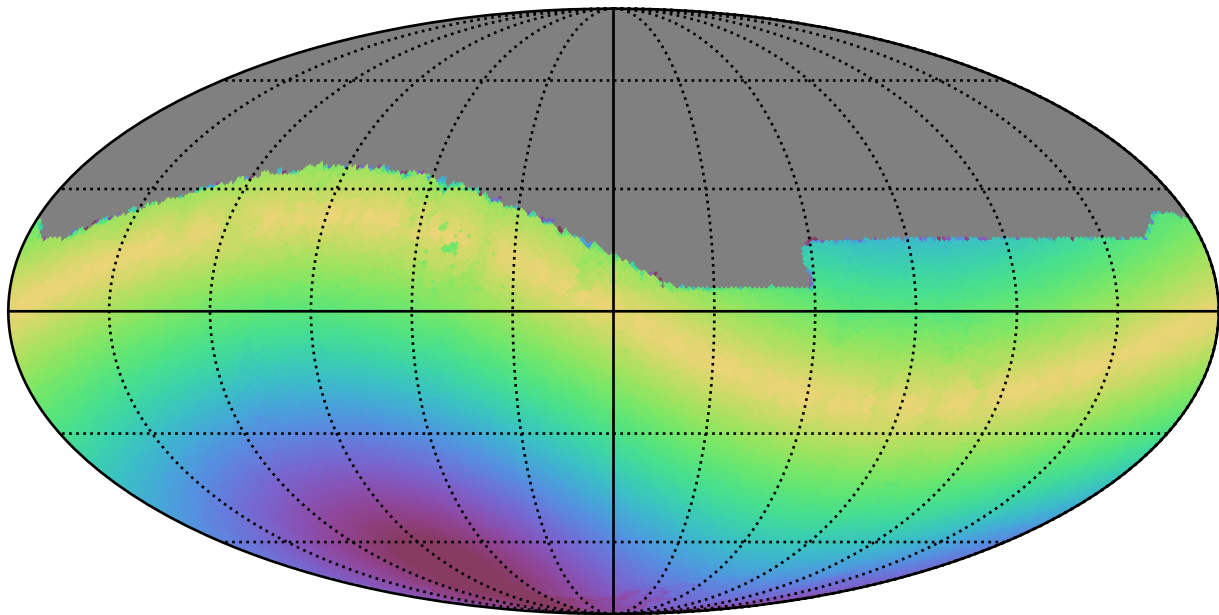
no_high_blob_v3.3_10yrs All sky z band: Max solarElong
