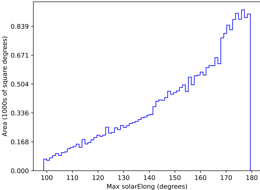
no_high_blob_v3.3_10yrs All sky z band: Max solarElong
