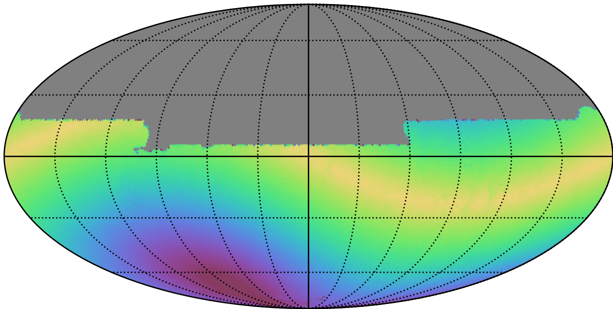
no_high_blob_v3.3_10yrs All sky y band: Max solarElong
