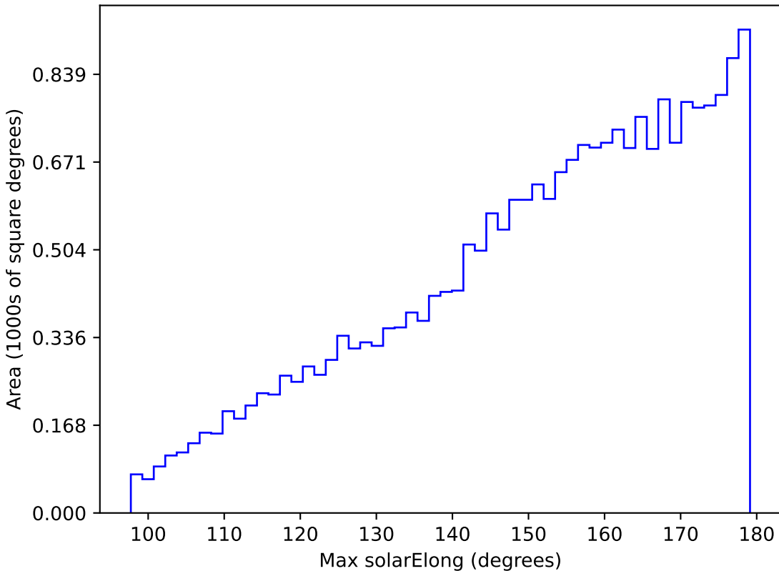
no_high_blob_v3.3_10yrs All sky y band: Max solarElong
