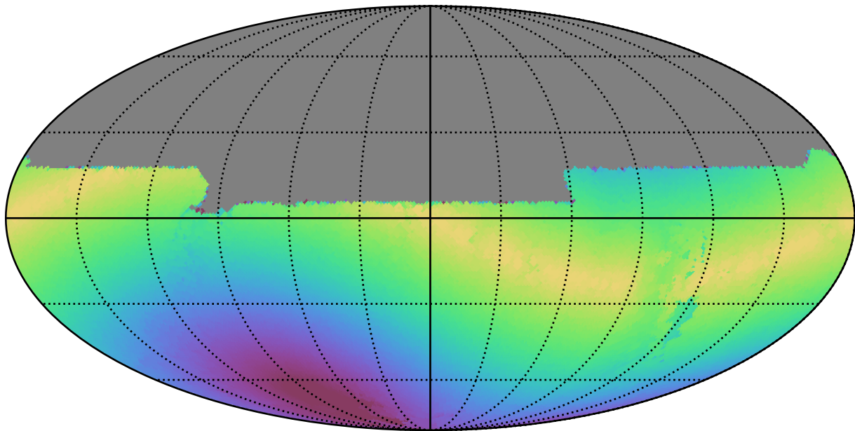
no_high_blob_v3.3_10yrs All sky u band: Max solarElong
