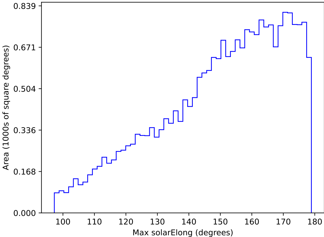
no_high_blob_v3.3_10yrs All sky u band: Max solarElong
