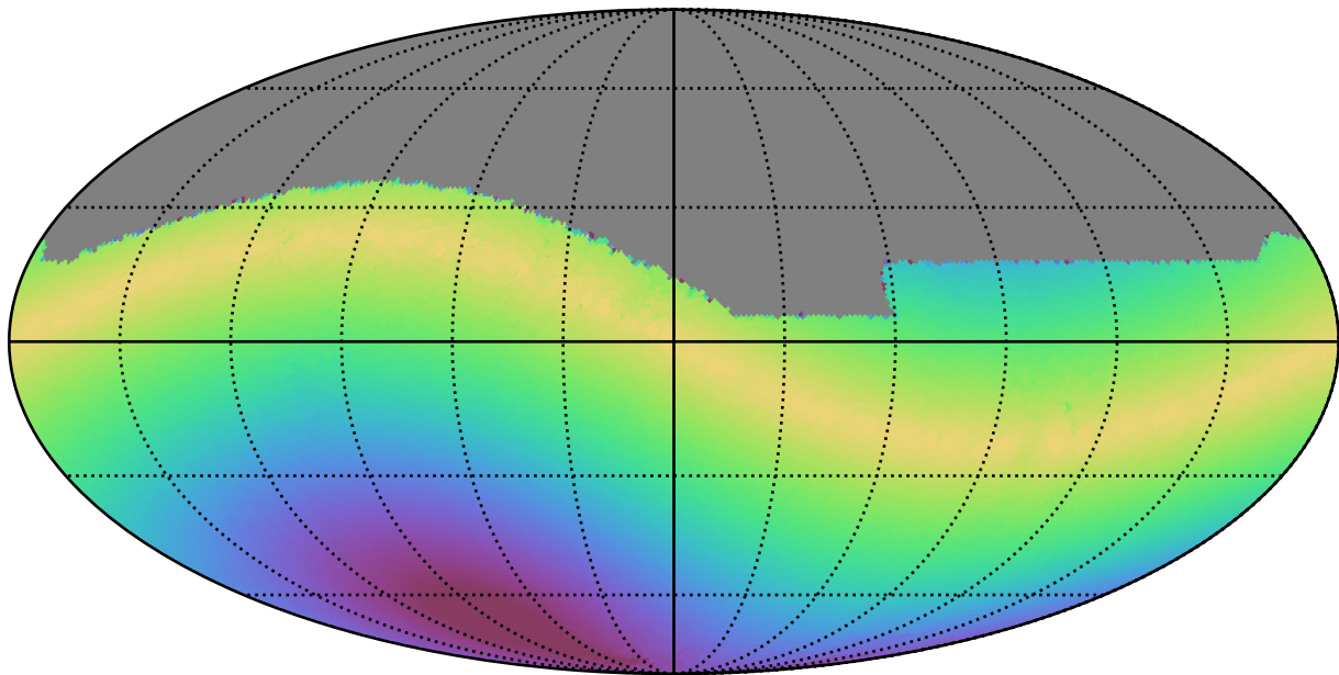
no_high_blob_v3.3_10yrs All sky r band: Max solarElong
