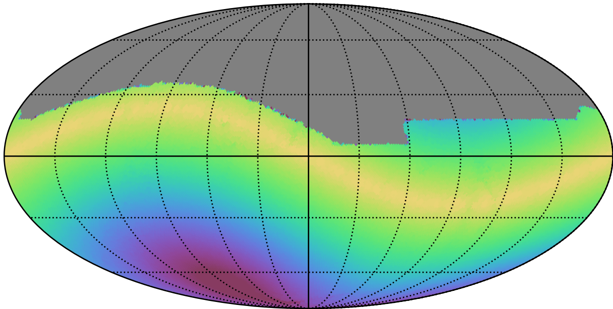
no_high_blob_v3.3_10yrs All sky i band: Max solarElong
