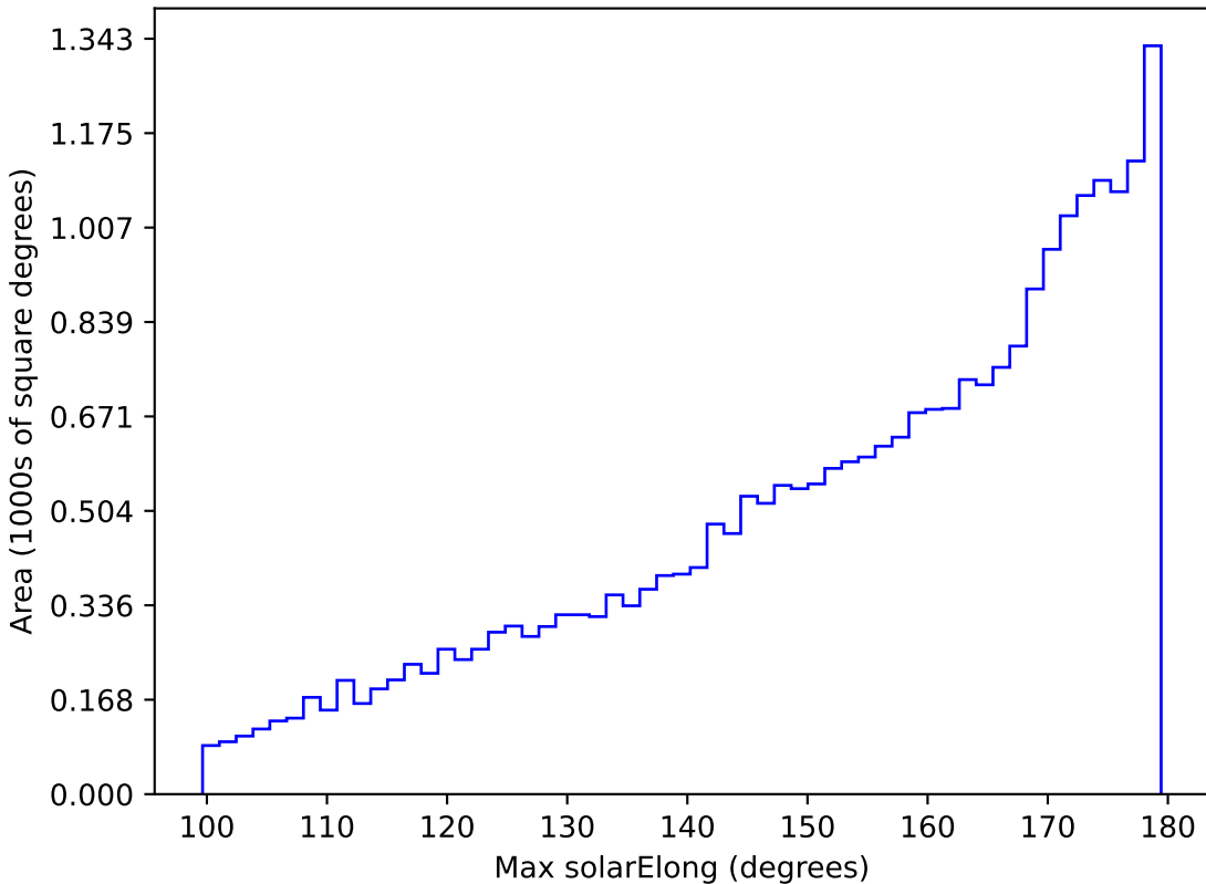
no_high_blob_v3.3_10yrs All sky i band: Max solarElong
