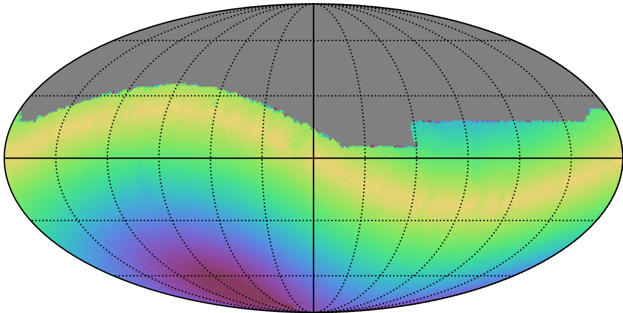
no_high_blob_v3.3_10yrs All sky g band: Max solarElong
