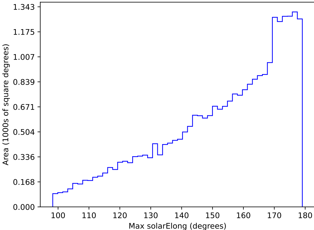
no_high_blob_v3.3_10yrs All sky g band: Max solarElong
