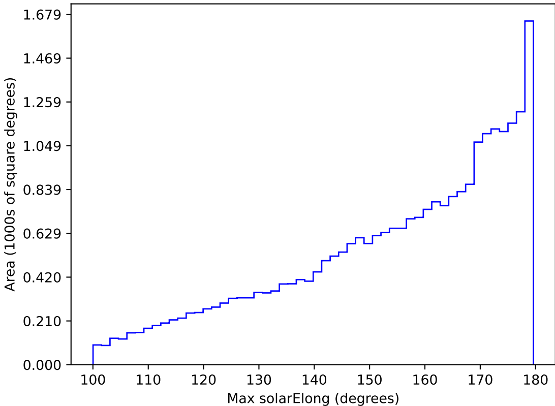
no_high_blob_v3.3_10yrs All sky all bands: Max solarElong
