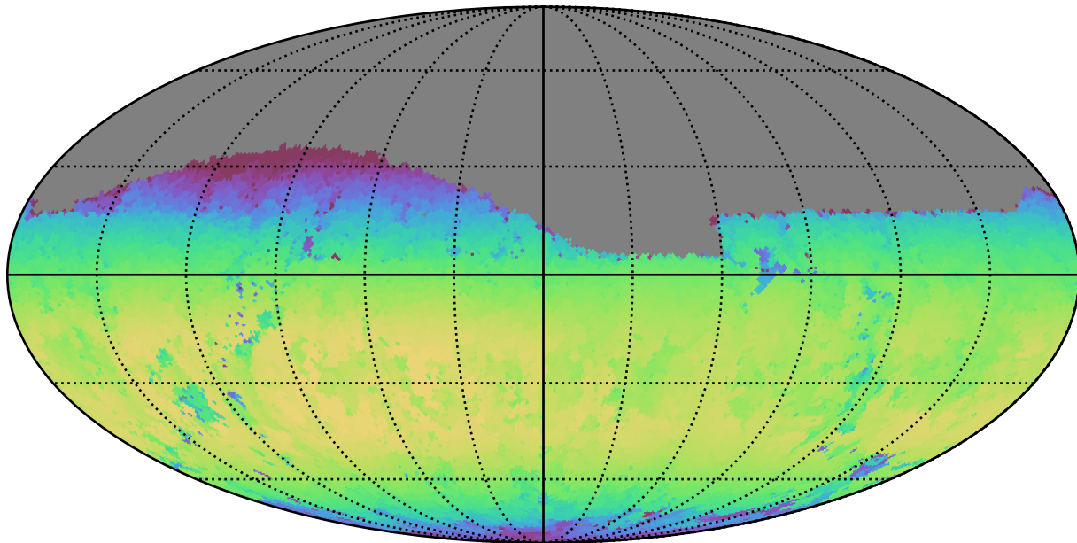
no_high_blob_v3.3_10yrs Yr 1 z band: Max skyBrightness
