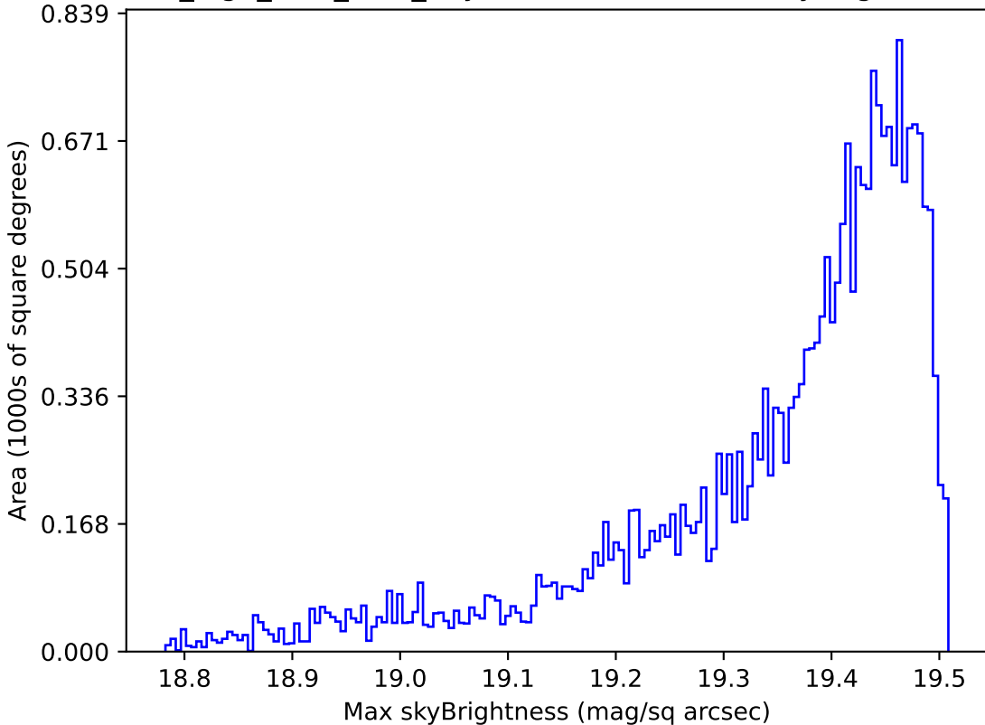
no_high_blob_v3.3_10yrs Yr 1 z band: Max skyBrightness
