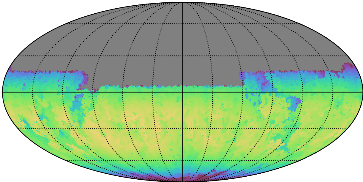
no_high_blob_v3.3_10yrs Yr 1 y band: Max skyBrightness
